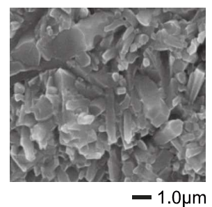
SEM Image of a section of sintered SN-E10
